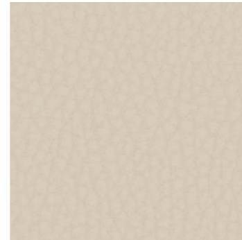
5187 Milky Way
