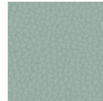
5216 Mercury's Albedo
