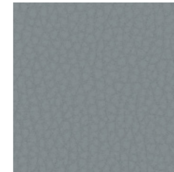
5192 Green Comet
