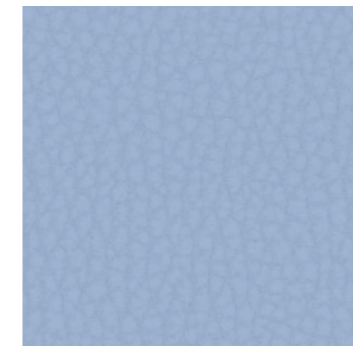
5191 Neptune Cloud
