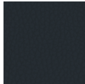
5190 Outer Space
