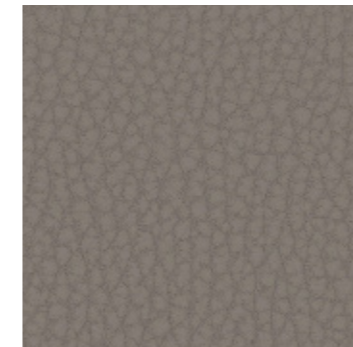
5198 Meteorite
