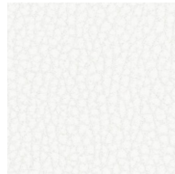
2769 Saturn's Moon
