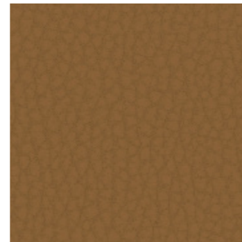
5197 Solar Wind
