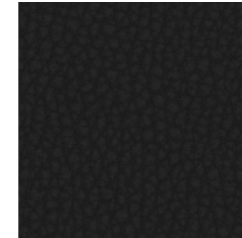
0565 Monolith
